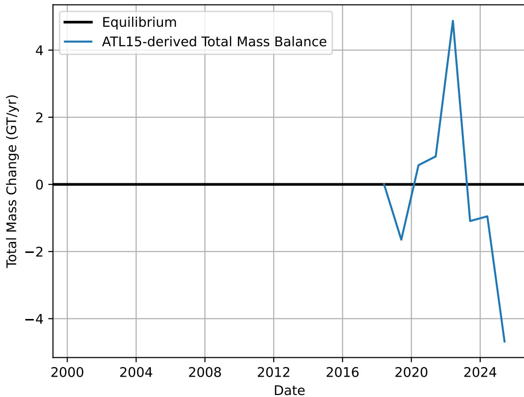
ATL15-derived Total Mass Balance
